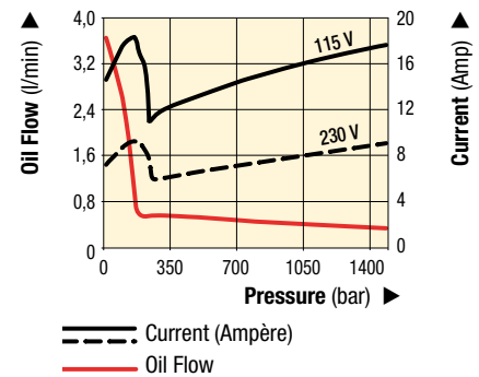
OIL FLOW VERSUS PRESSURE
